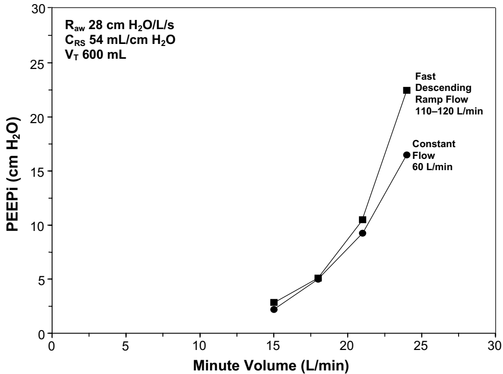
Fig. 7. Intrinsic positive end-expiratory pressure (PEEP) with constant and descending ramp inspiratory flow and equal duty cycles. R_{aw} = airway resistance (28 cm H 2 O/L/s). C_{RS} = compliance of the respiratory system (54 mL/cm H 2 O). V_T = tidal volume (600 mL).
