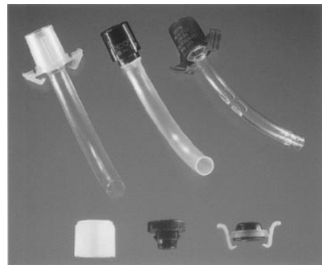
Fig. 19. Examples of decannulation caps (below) and associated inner cannulae (above). (Courtesy of Tyco Healthcare, Pleasanton, California.)
