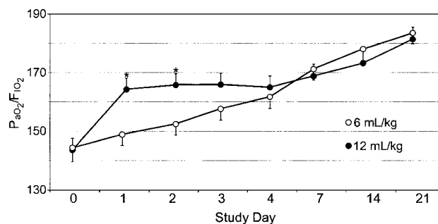
Fig. 1. The ratio of P_{aO_2} to fraction of inspired oxygen ( P_{aO_2}/F_{IO_2} or P/F) in the patients in the small- V_T (6 mL/kg) and large- V_T (12 mL/kg) groups over the duration of the ARDS Network V_T trial. 19 Note that the large V_T strategy produced a better ratio (presumably from less fixed atelectasis) over the first few days of the trial (* = p < 0.05 ), even though the ultimate outcome was worse. (Data from Reference 19.)
