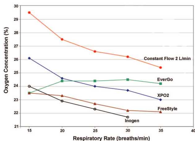
Fig. 7. Effect of breathing frequency on fraction of inspired oxygen with continuous flow at 2 L/min, with 4 pulse-dose-only portable oxygen concentrators at the numerical setting of 2. (Adapted from Reference 57.)
