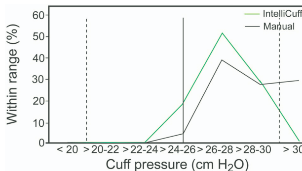
Fig. 5. This graph shows the percentage of total time cuff pressure recordings were within each range during 8 h of ventilation without movement for both the IntelliCuff and manual technique. Each recording corresponds to an average cuff pressure during 3 s of ventilation. A higher curve denotes a higher frequency of cuff pressure observations within that range. The total number of observations is the same for the 2 techniques and includes all tested scenarios in the second part of the study. The initial set cuff pressure was 25 cm H 2 O, as shown by the solid vertical line in the middle. The outer dashed lines depict the edges of the generally accepted cuff pressure range of 20–30 cm H 2 O.
