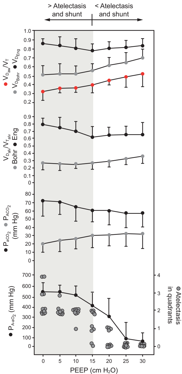
Fig. 2. Gas exchange and performance of the Bohr and Engghoff parameters as a function of PEEP, which was used as a surrogate of shunt. Atelectasis was diagnosed with lung ultrasound. Cumulative presence of atelectasis of all quadrants (ventral and dorsal, right and left) of all animals is presented as circles for each level of PEEP. A circle at zero means that the animal did not develop atelectasis. Analysis of variance was used for all variables ( P < .001 ). V_{DBohr} and V_{DEng} = physiological dead space using the Bohr and Engghoff formulas, respectively; V_{Daw}/V_T = airway dead space; V_{Dalv}/V_{T_{alv}} = ratio of alveolar dead space to alveolar tidal volume; P_{ACO_2} = alveolar P_{CO_2} . P_{(A-a)O_2} = alveolar-arterial O_2 difference.
