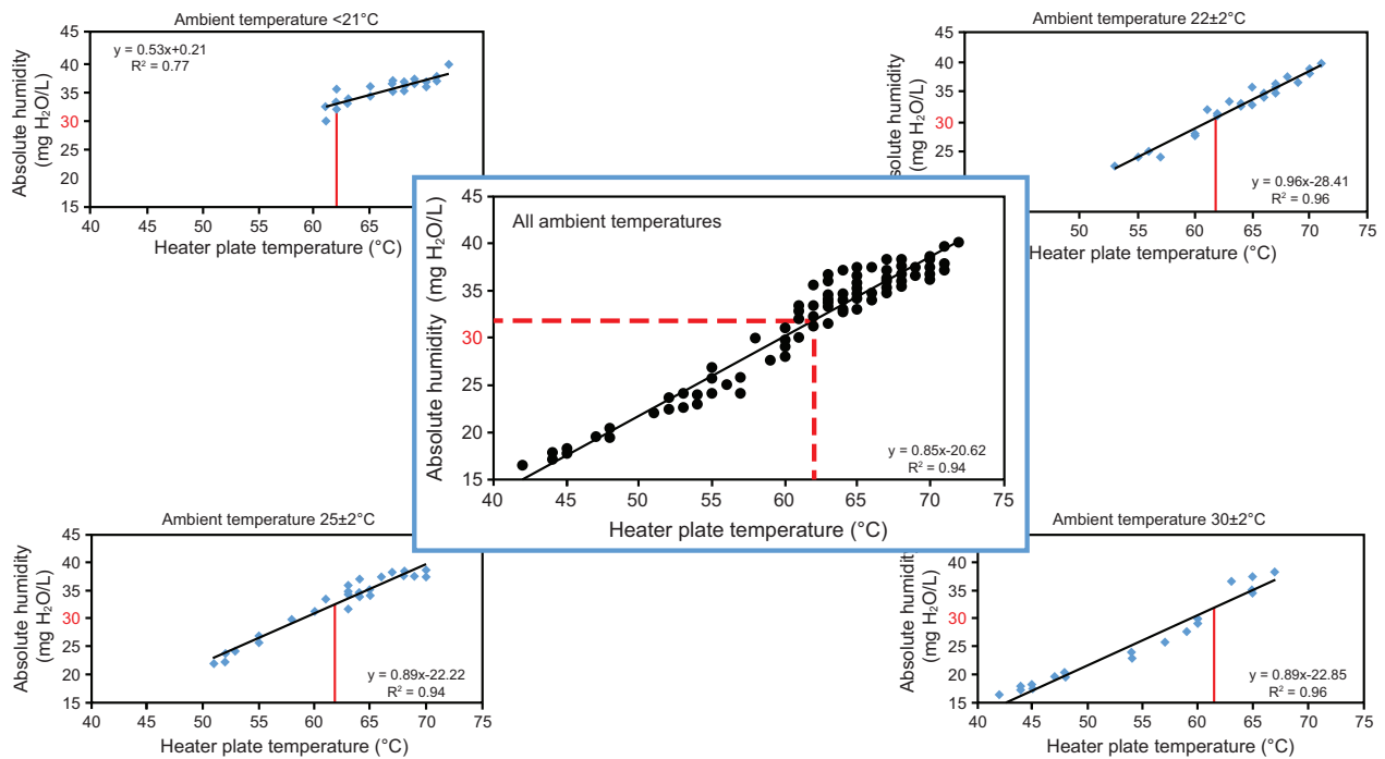
Fig. 3. Relation between the heater plate temperature (in °C) and absolute humidity (mg H 2 O/L) with an MR850 heated-wire heated humidifier. We conducted a bench study including 105 measurements of absolute humidity at steady state (after 1 h of stability) with the psychrometric method, 20 with varying the heater plate temperature. We found a strong correlation between the heater plate temperature and the delivered inspiratory absolute humidity ( R^2 = 0.9425 , P < .001 ). Data for different ambient temperatures (below 21°C, 22 ± 2°C, 25 ± 2°C, and 30 ± 2°C) are displayed, and the central panel shows all data. A heater plate temperature > 62°C ensures a safe humidity delivered whatever the ambient temperature.
